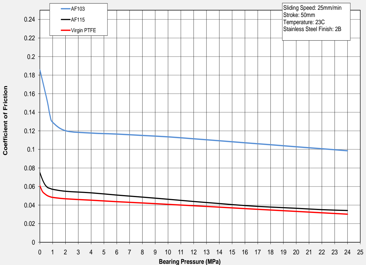
Effect of Load on Frictional Coefficient for various materials
